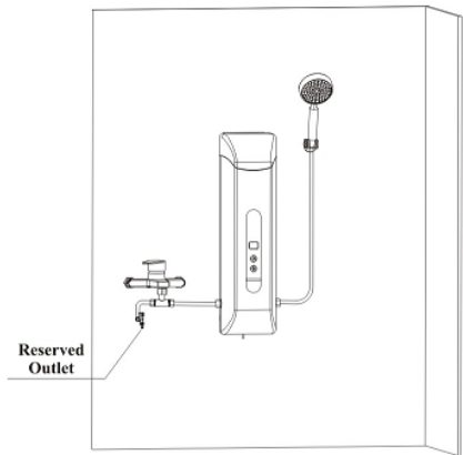
( Figure 8 ) Installation Schematic View of Shower Softener at the Right Side of Water Mixing Valve with Spare Outlet Reserved
