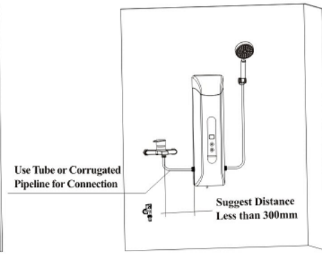
( Figure 7 ) Installation Schematic View of Shower Softener at the Right Side of Water Mixing Valve
