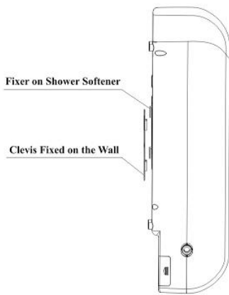
( Figure 2 ) The Shower Softener Fixed on the Wall
