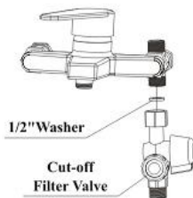
( Figure 14 ) Installation of Cut-off Filter Valve
